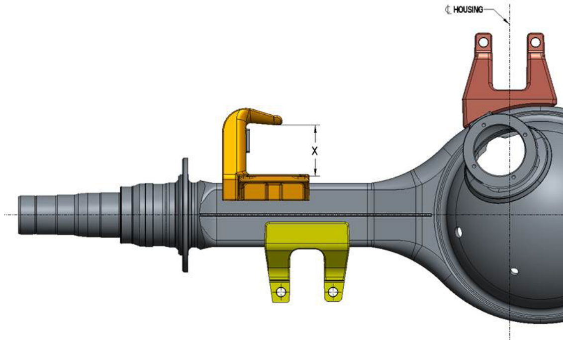
Figure 1: Illustration of spring saddle bracket to suit 6 Rod suspensions.
